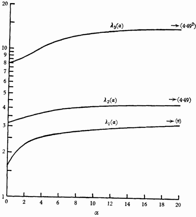
FIGURE 1. Principal eigenvalues for problem 6.
