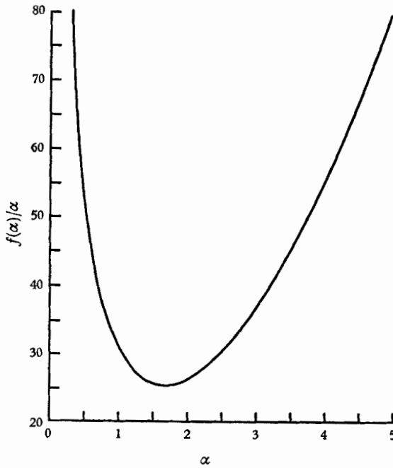
FIGURE 2. Graph of f(\alpha)/\alpha as given by equation (11). In the boundary layer no linear disturbance can exist if qR is in the region below the graph.
